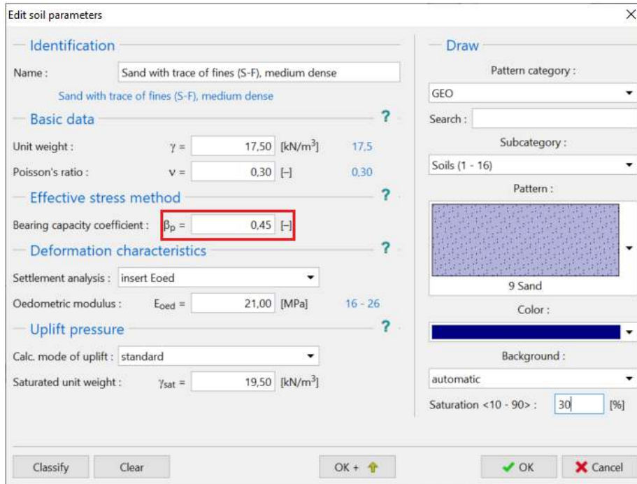
Dialog window “Edit soil parameters” – soil S-F
