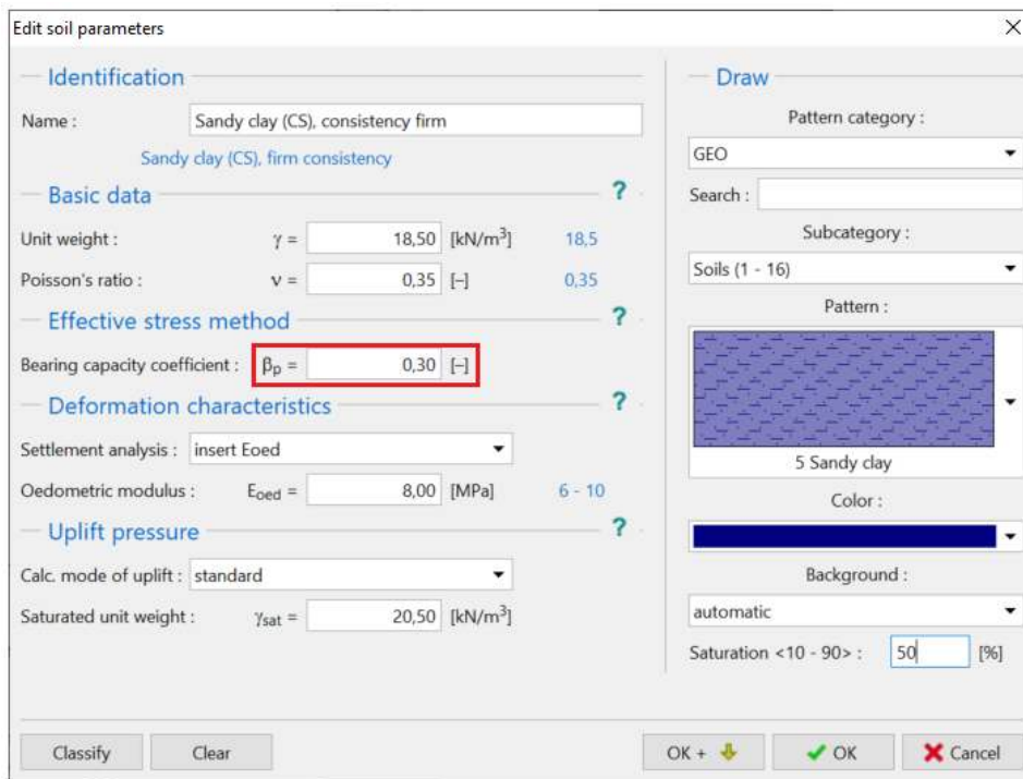
“Edit soil parameters” Dialog window – soil CS
