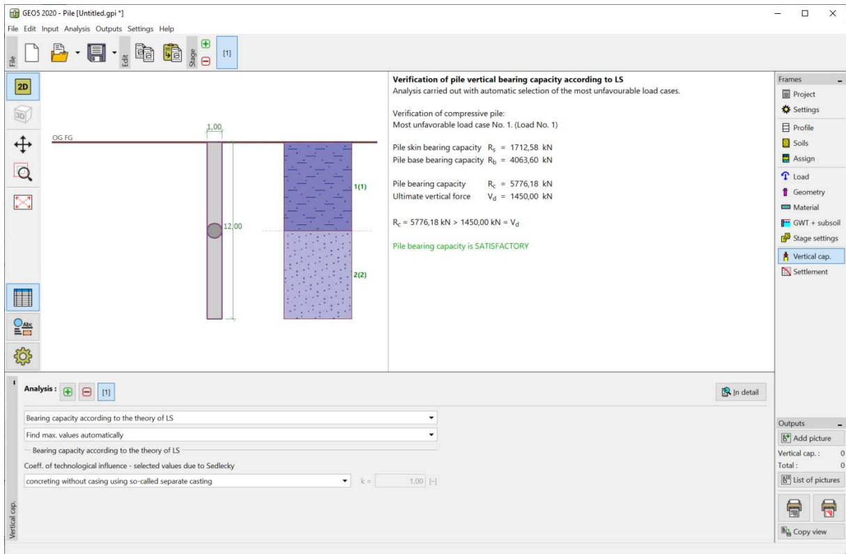
“Vertical capacity – assessment according to CSN 73 1002” frame
