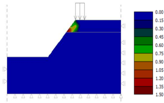
Figure 20: Contours of the equivalent plastic strain for slope of layered soil with surcharge by FEM ( \beta = 45^\circ and h/t = 0 )
