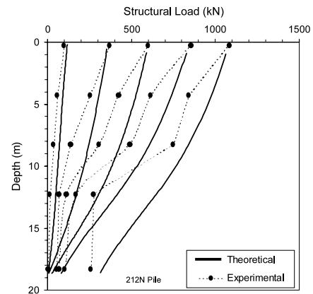
Fig. 7. Load transfer curve 212N pile.
